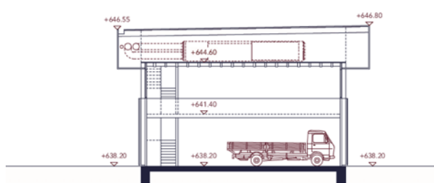
Querschnitt Facility Management
