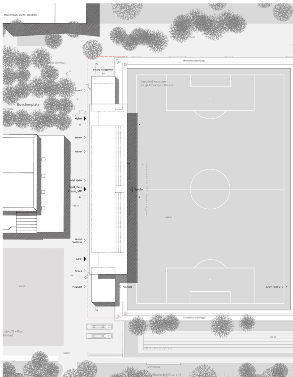
Situation
